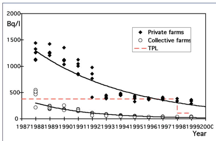
FIG. 5. Reduction with time of ^{137}\text{Cs} activity concentration in milk produced in private and collective farms of the Rovno region of Ukraine with a comparison to the temporary permissible level (TPL).
