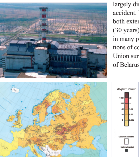
FIG. 1. Surface-ground deposition of 137 Cs throughout Europe as a result of the Chernobyl accident (De Cort et al. 1998).
