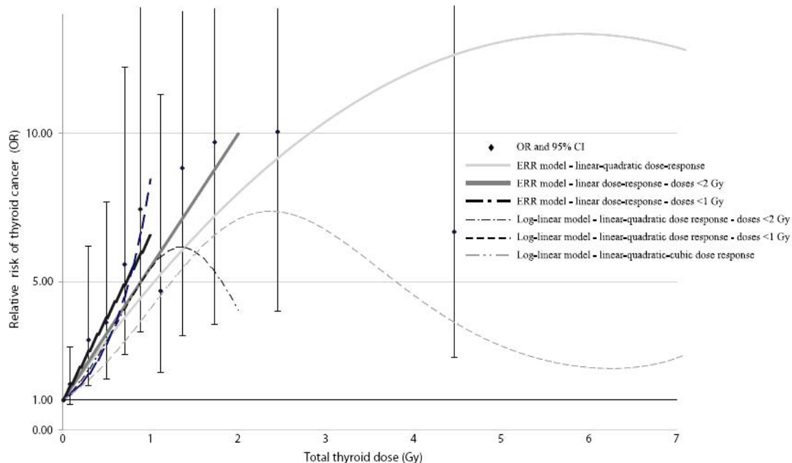
Figure 6.2. Comparison of relative risks predicted by the different risk models (ERR and log-linear over the entire dose range and in restricted doses ranges) with categorical relative risk estimated in 11 dose categories (from Cardis et al. , 2005)
